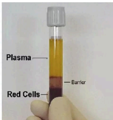
Figure 1. Plasma, barrier and red cells
